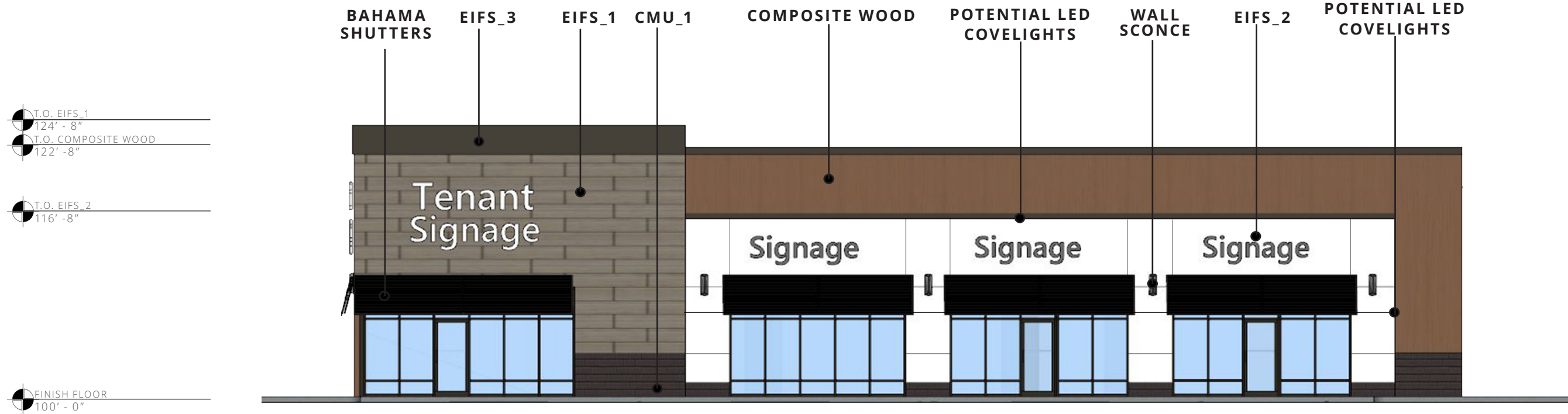
FRONT ELEVATION
