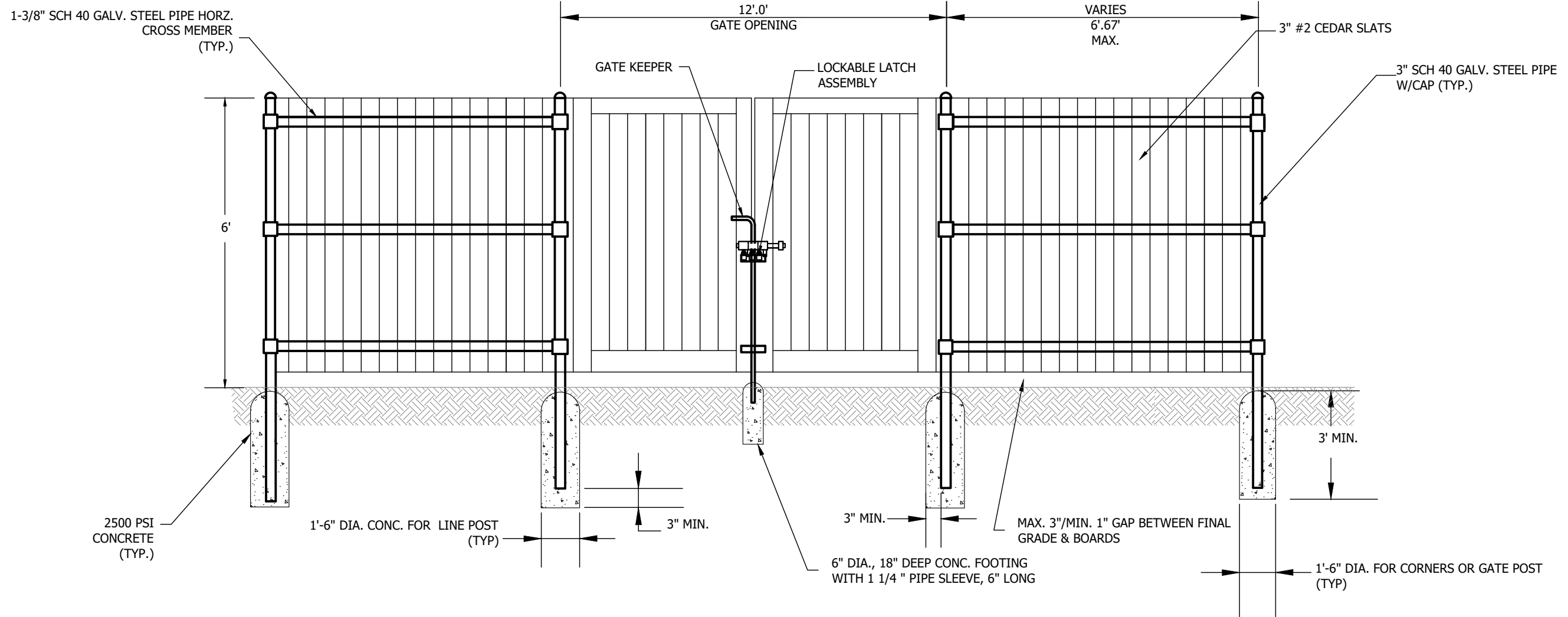
1 TYPICAL 6' WOOD FENCE DETAIL SCALE: N.T.S.
