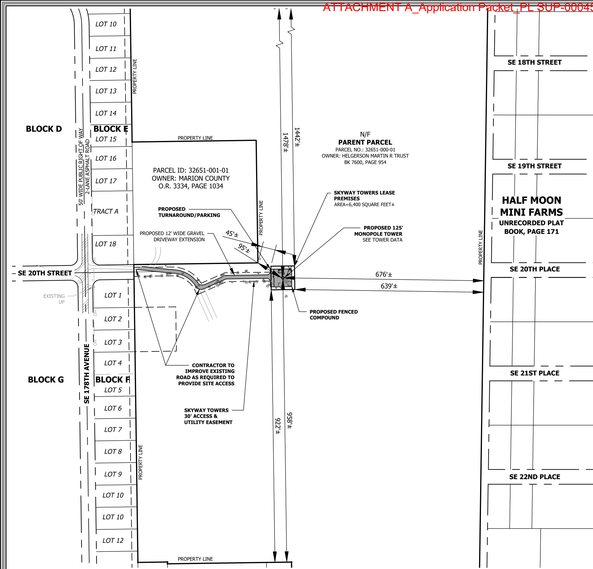
1 OVERALL SITE PLAN SCALE: 1" = 200' 0' 100' 200' 300' 400'
