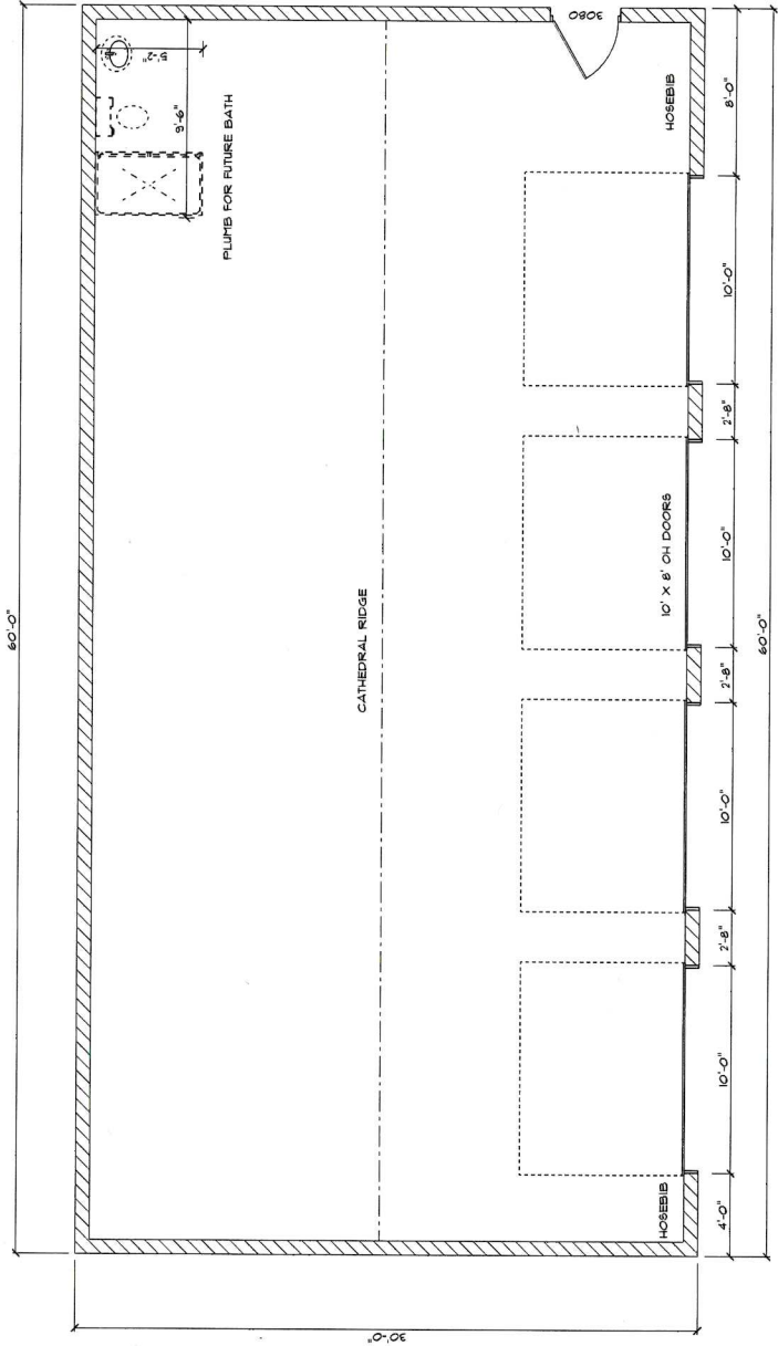
SHOP FLOOR PLAN SCALE: 1/4" = 1'-0" 1800 SF SHOP
