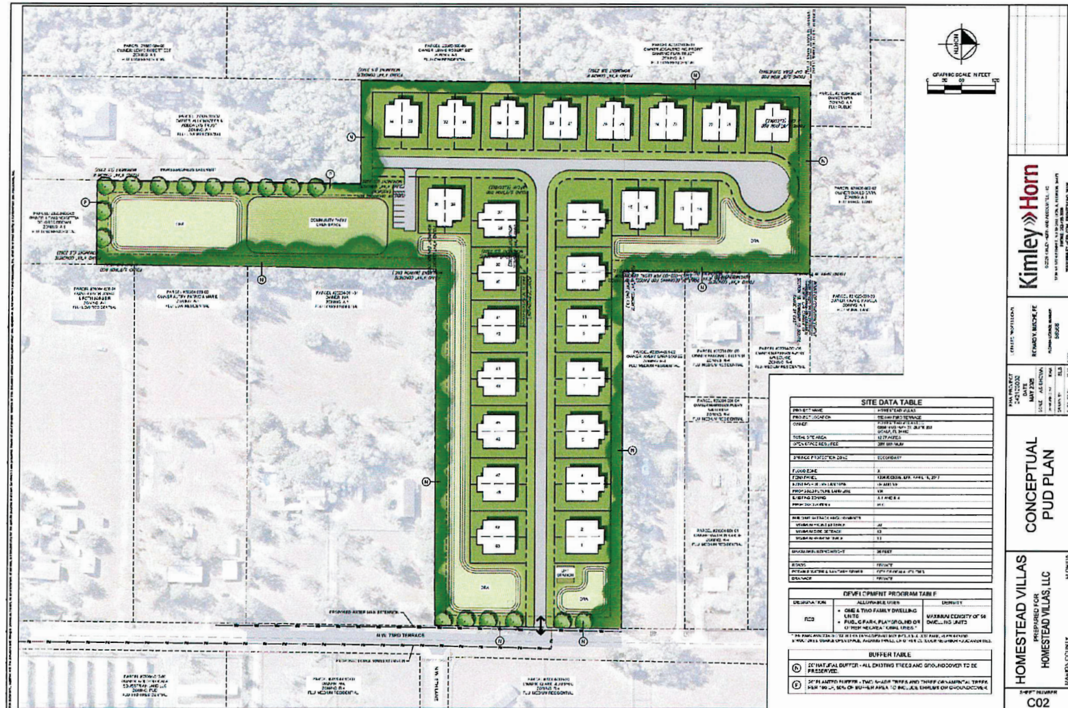
Figure 1: Homestead Villas Conceptual PUD Plan
